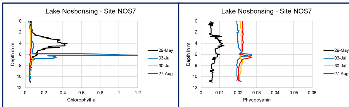
Figure 14. Algal pigments in West Basin.
