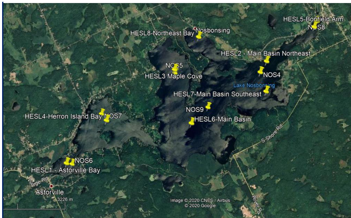
Figure 4. Sample Sites in Lake Nosbonsing. “HESL” denotes Lake Partner, “NOS” denotes NBMCA.
