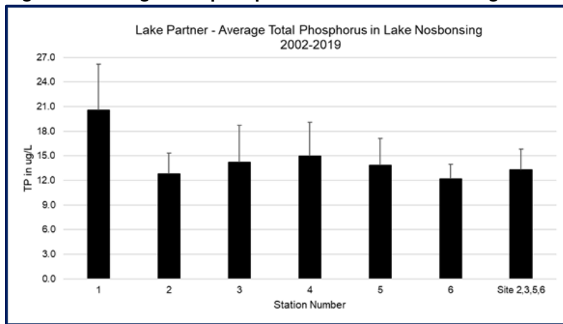
Figure 5. Average total phosphorus in Lake Nosbonsing : 2003 – 2019.
