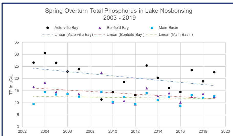
Figure 6. Total Phosphorus Trends in Lake Nosbonsing : 2003 – 2019.
